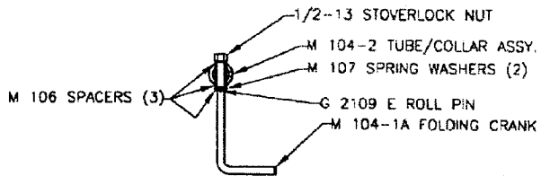
M 104 A FOLDING CRANK DETAIL
