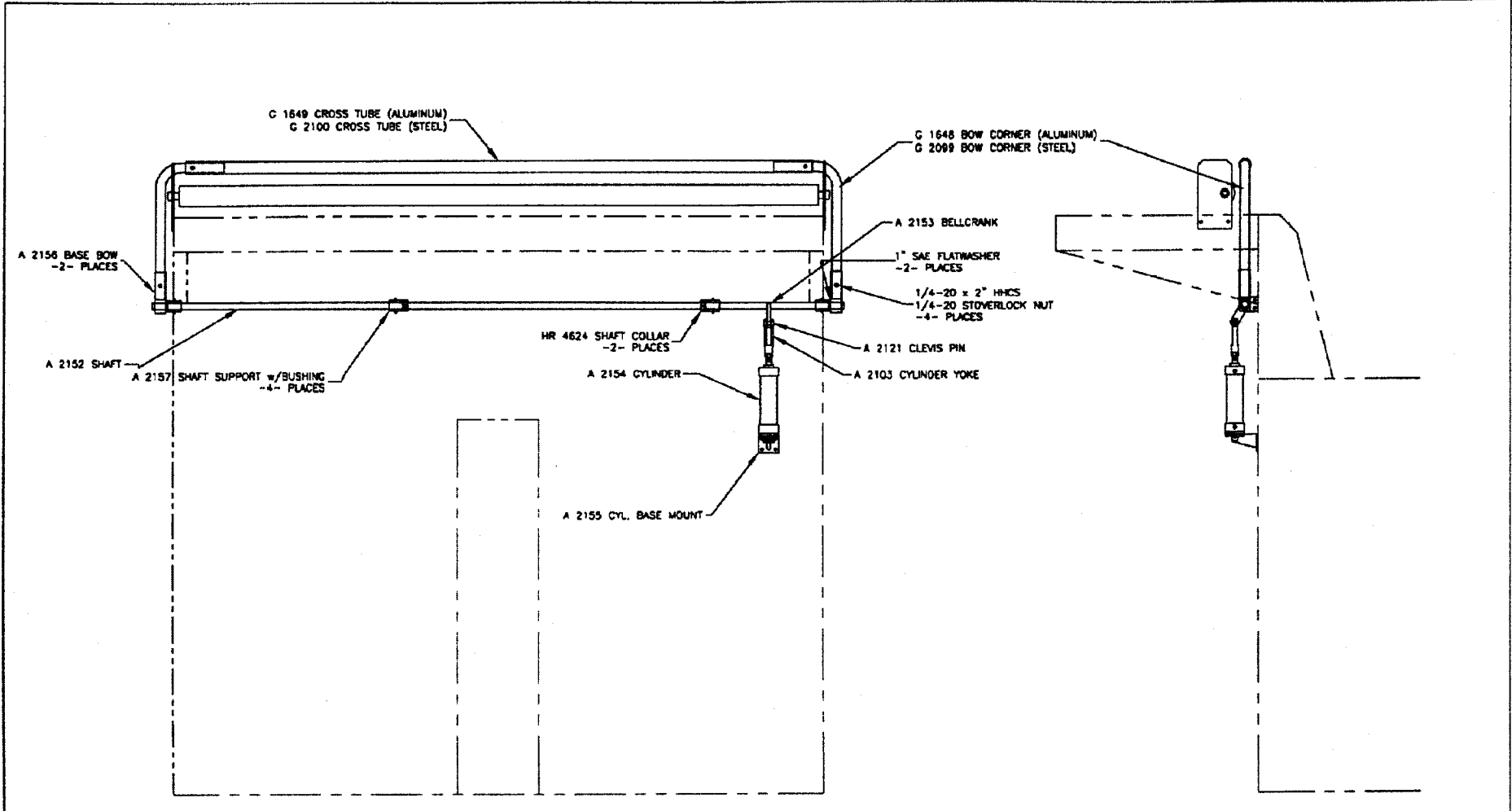
VIEW FROM FRONT OF BODY
