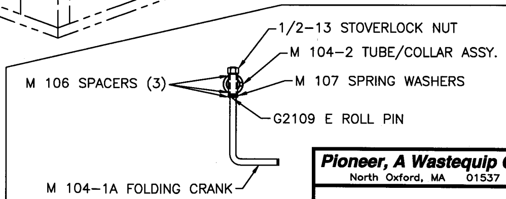
FOLDING CRANK - PARTS DETAIL M 104 A
